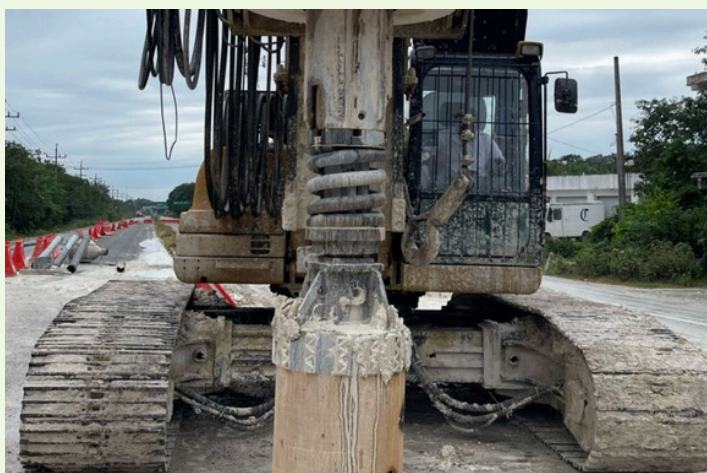
RIGID INCLUSIONS
